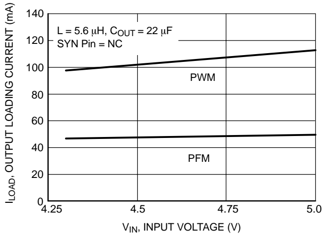
Figure 14. PWM/PFM Switchover Current Thresholds vs. Input Voltage ( V_{OUT} = 3.3 V)
